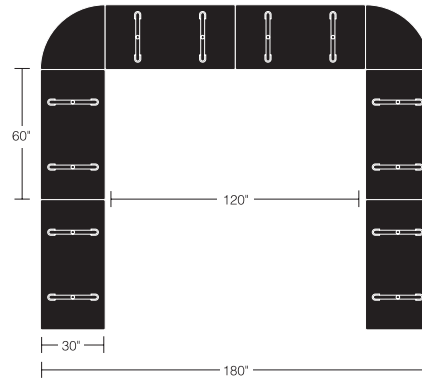
Six rectangles 60" x 30" Two 90° wedge connecting tops Seating capacity - 14 2 ganger kits provided with each wedge connecting top Order three additional ganger kits
