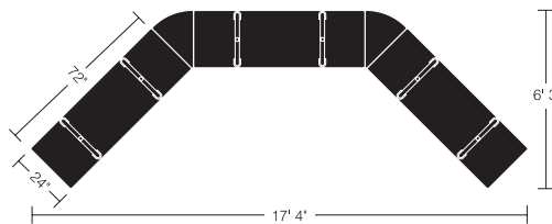
Three rectangles - 72" x 24" Two 45° wedge connecting tops Seating capacity - 8 Two ganger kits provided with each 45° wedge connecting top
