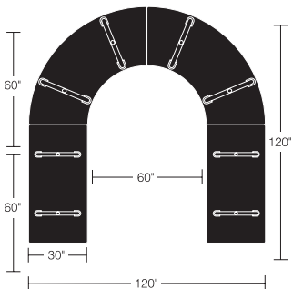
Two 90° arc connecting tops Two 60" x 30" rectangles Seating Capacity - 10 2 ganger kits provided with each 90° arc
