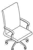
Overall: 26½"D 26½"W 46"-49"H Inside: 19"D 21½"W 18½"H Seat: 18½"-21½"H Arm: 25¾"-28¾"H
