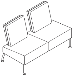
Overall: 27"D 49"W 30½"H Inside: 17"D 49"W 18"H Seat: 17"H Arm: 21"H
